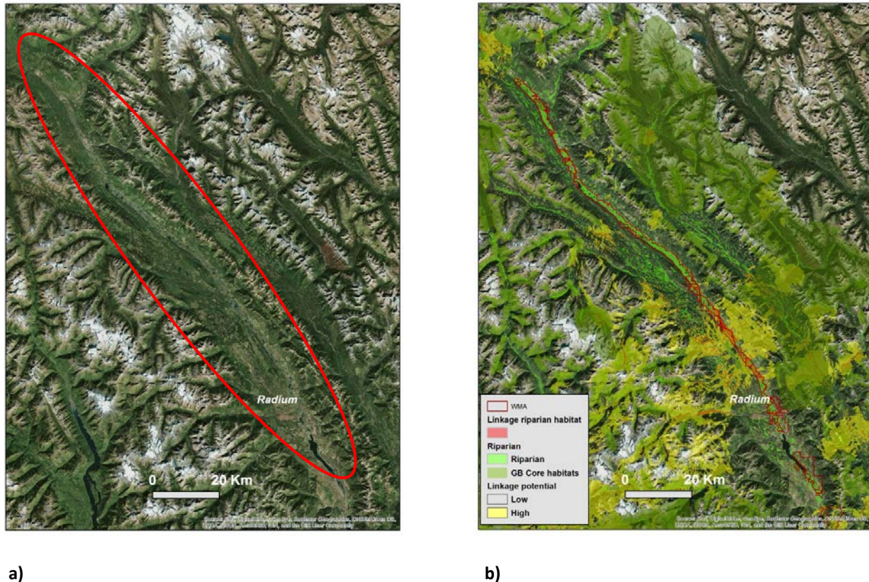
Figure 8. a) Google Earth image of the Columbia Wetlands north-south along the Rocky Mountain Trench (red oval) and with east-west corridors connecting the Purcell and Rocky Mountains along BC Highway 95 north of Radium, BC; and b) the same area with grizzly bear core (green) and linkage (yellow) habitats overlaid with riparian-wetland habitats (orange) in the valley bottom.
