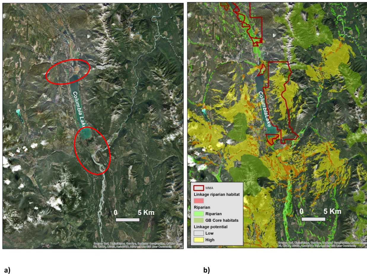
Figure 9. a) Google Earth image of the Columbia Lake Wetlands corridors (red ovals) connecting the Purcell and Rocky mountains along BC Highway 95 near Canal Flats, BC; and b) the same area with grizzly bear core (green) and linkage (yellow) habitats overlaid with riparian-wetland habitats (orange) in the valley bottom.
