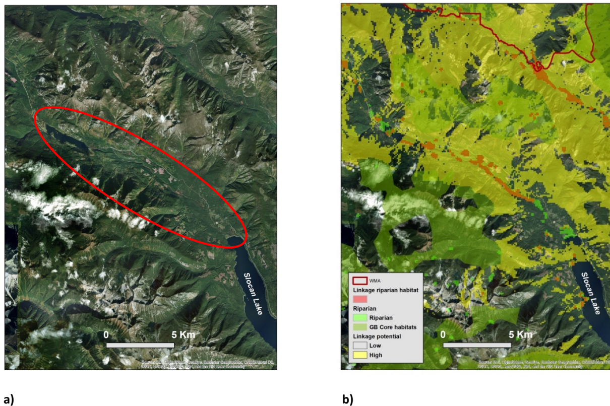
Figure 7. a) Google Earth image of the Bonanza Biodiversity Corridor (red oval) extending along BC Highway 6 between Slocan and Summit Lakes connecting the Valhalla and Selkirk mountain ranges; and b) the same area with grizzly bear core (green) and linkage (yellow) habitats overlaid with riparian-wetland habitats (orange) in the valley bottom.
